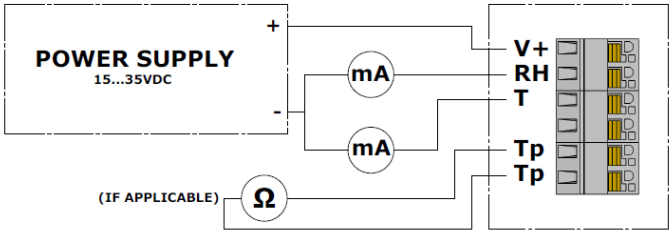
Fig. 3. Connection diagram, current output
